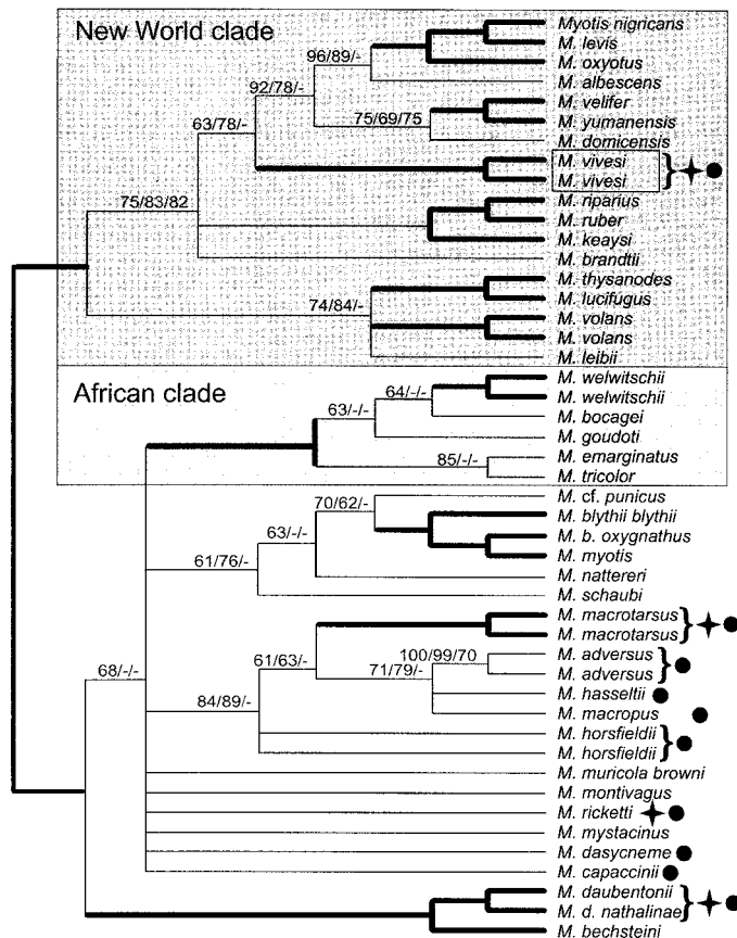
FIG. 2. —Same legend as in Fig. 1, but analyses restricted to Myotis species only, with the addition of 5 partial cytochrome- b ( Cytb ) gene sequences (for M. leibii , 2 M. adversus , M. macropus , and M. horsfieldii ).
